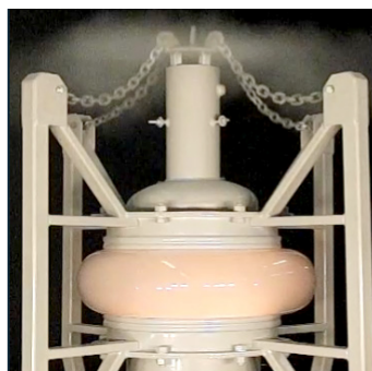
EXPLOSION TESTING
